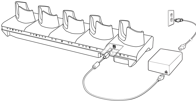
Figure 41 Connect Charge Only Cradle Power
