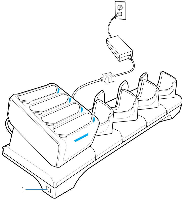
Figure 39 4-Slot Charge Only Cradle with Battery Charger
