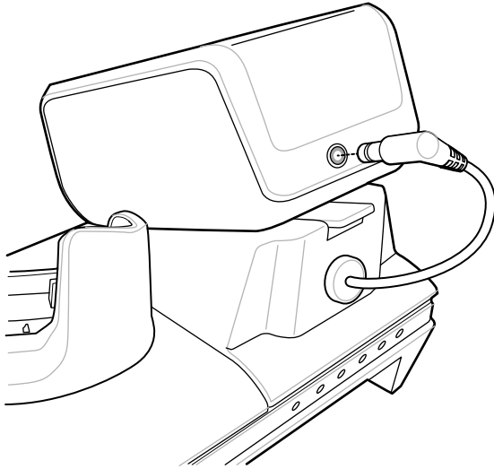
Figure 41 Connect Charge Only Cradle Power
