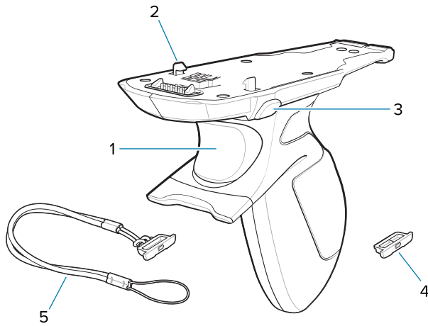
Figure 48 Trigger Handle
