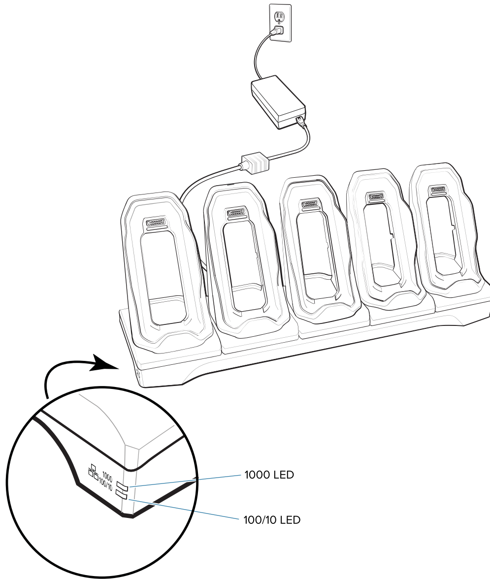
Figure 42 5-Slot Ethernet Cradle
