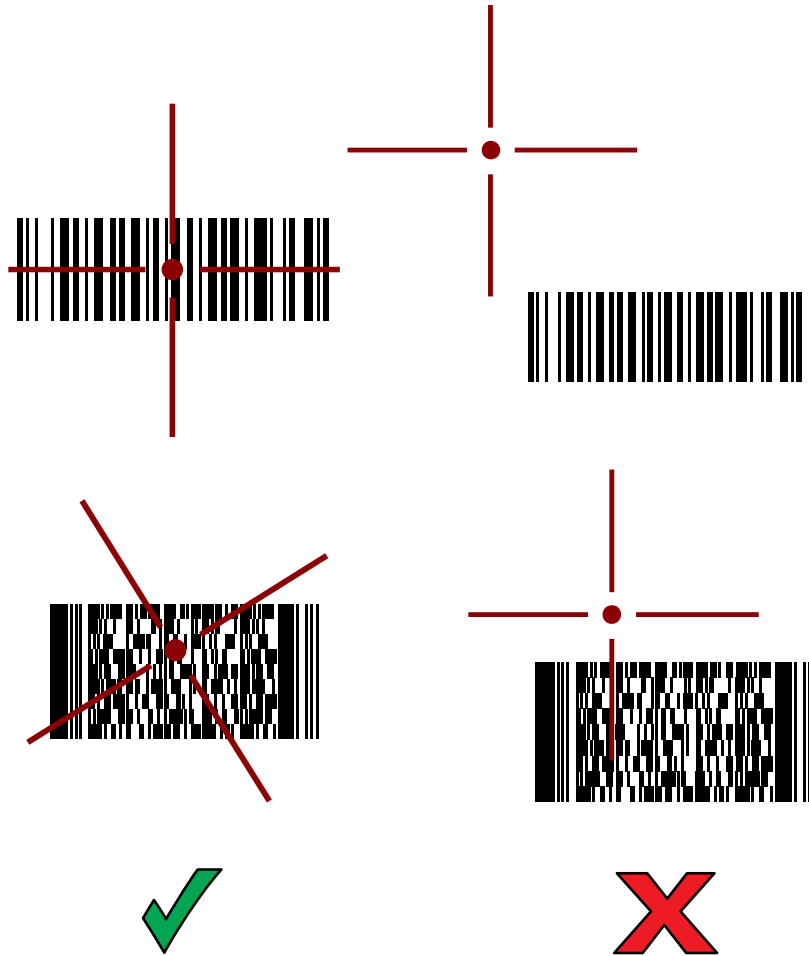
Figure 12 Aiming Pattern: Standard Range
